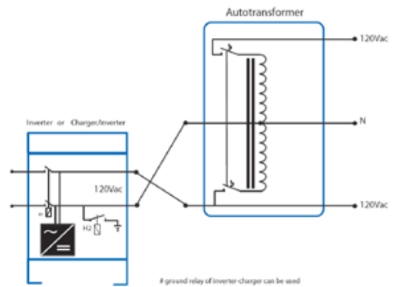
Autotransformer: schematic diagram
